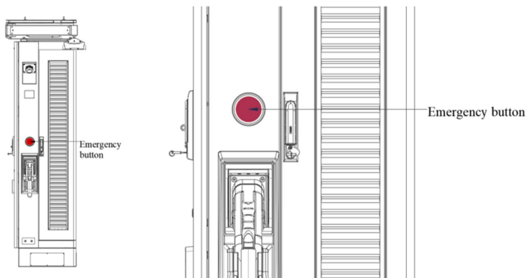
Figure 55. Emergency Stop Button
