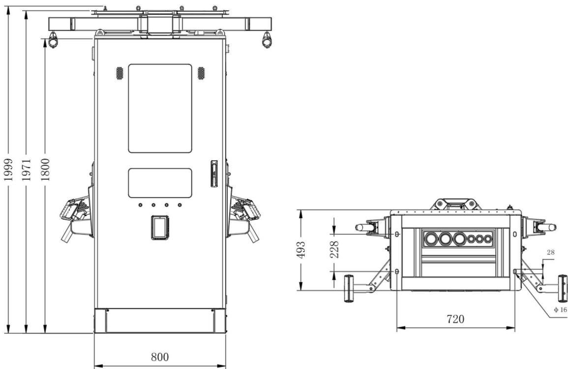
Figure 9. Installation Size
