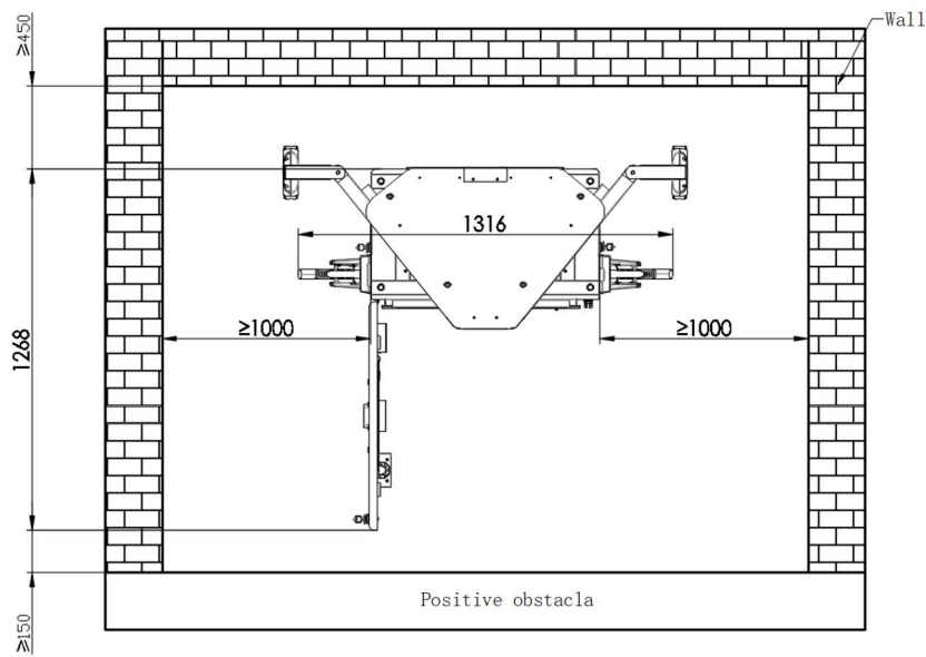
Figure 8. Maintenance Distance Diagram
