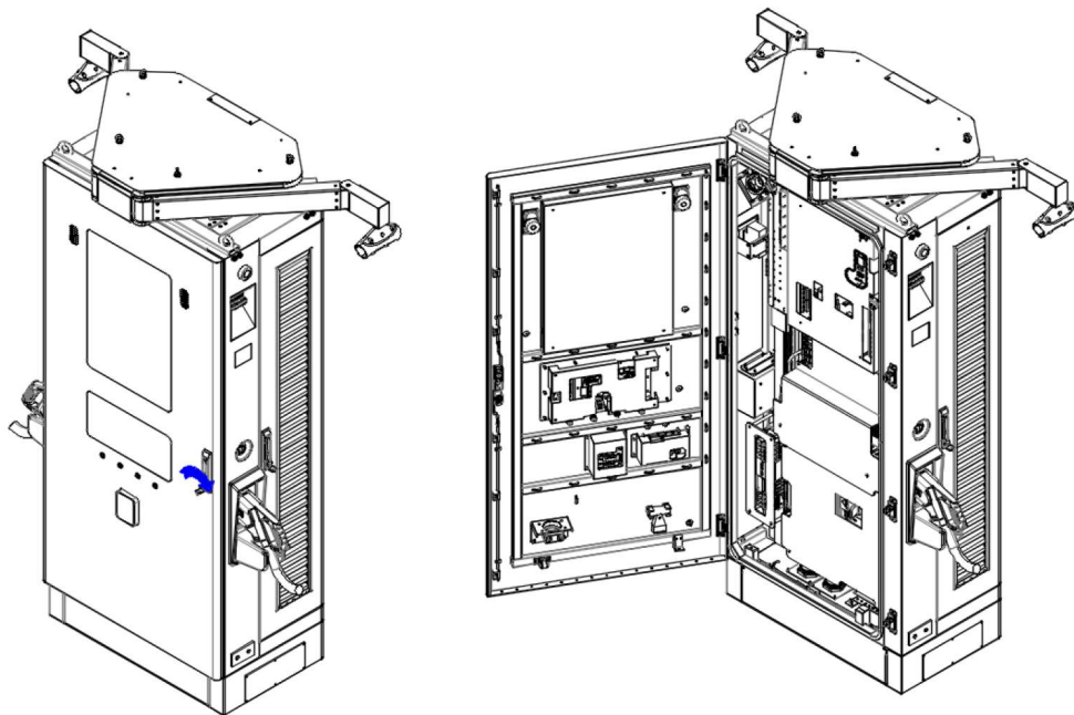
Figure 52. Open the EVSE Front Door
