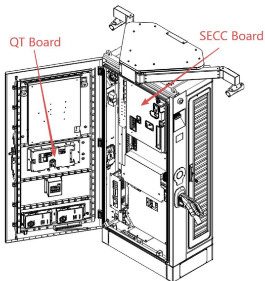
Figure 26. Control Board Location Diagram
