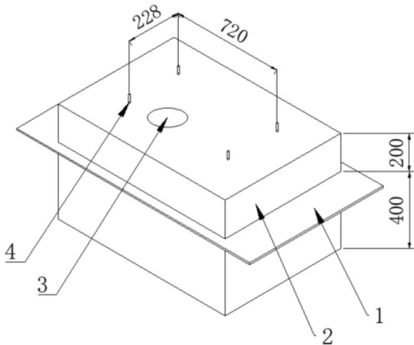
Figure 12. Schematic Diagram of Cement Foundation
