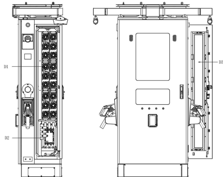
Figure 4. Right Component Diagram
