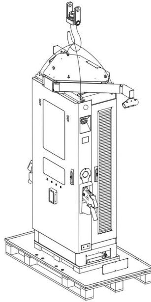
Figure 19. Lifting the EVSE with a Crane
