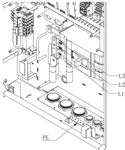
Figure 23. Wiring Diagram
