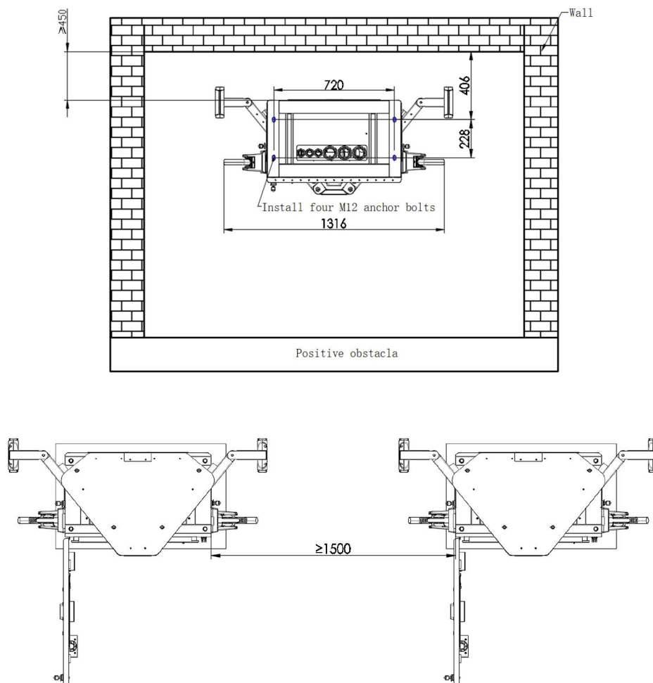
Figure 7. Installation Distance Diagram
