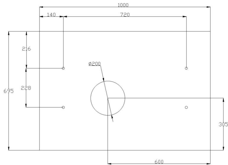
Figure 13. Plane dimensions of cement base of charging station
