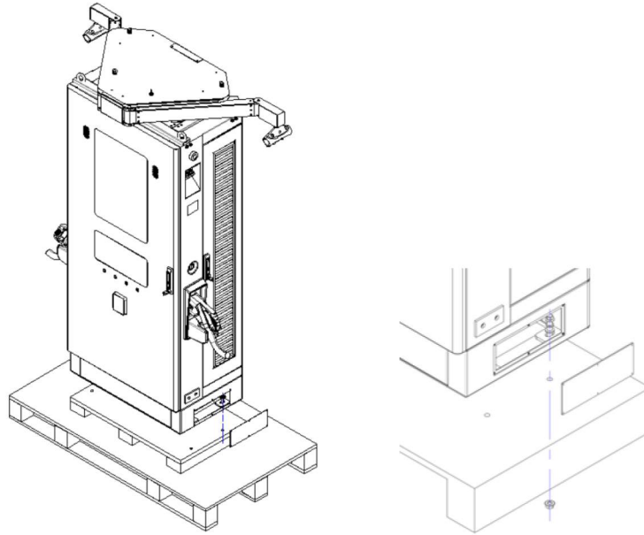
Figure 17. Diagram of Removing the Tray.
