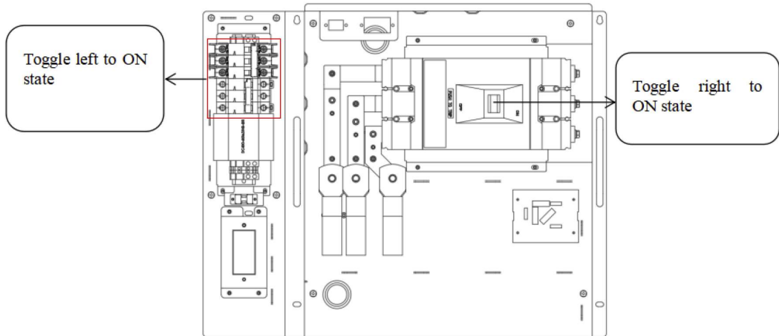
Figure 31. Switching On the Circuit Breaker, Leakage Protection and Air Switch
