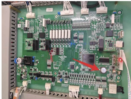
Figure 30.Battery Location Diagram(For SECC Board)
