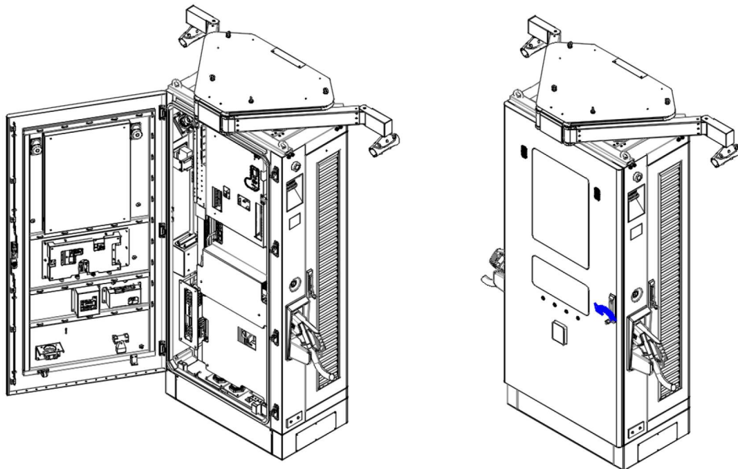
Figure 32. Close the Cabinet Door
